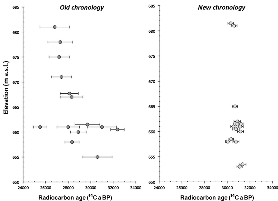
Figure 6. Comparison of the original Baumkirchen uncalibrated radiocarbon chronology (Fliri et al. , 1971, 1972; Fliri, 1976; Patzelt, 1996) and the new AMS-based chronology (this study). A few symbols were shifted by 0.5 m along the vertical axis to avoid overlapping error bars of replicates of the same elevation.
